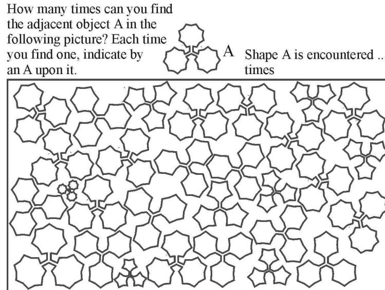
Figure 1: Form Analysis task FA1 (Scaled-down to 70% of the original)
