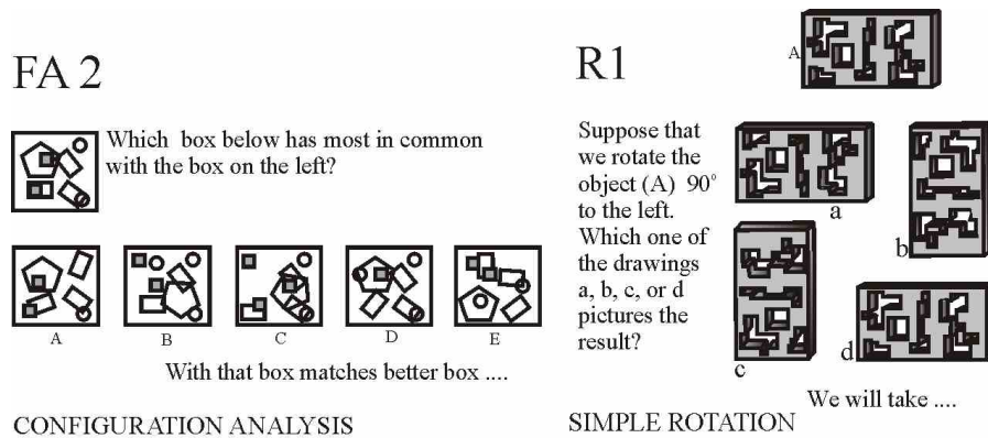
Figure 2: Configuration Analysis (FA2, left) and simple Rotation (R1, right) tasks (Scaled-down to 50% of the original)
